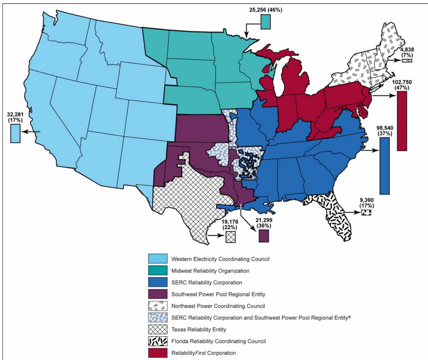
Figure 8: Capacity and Share of Total Capacity from Coal-Fueled Electricity Generating Units by Region, as of April 9, 2012
