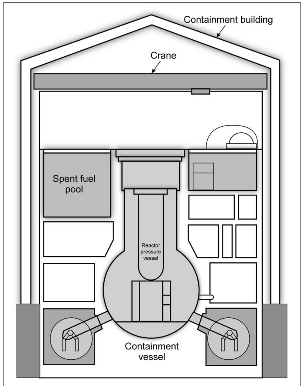
Figure 3: Location of a Spent Nuclear Fuel Pool in a Boiling Water Reactor
