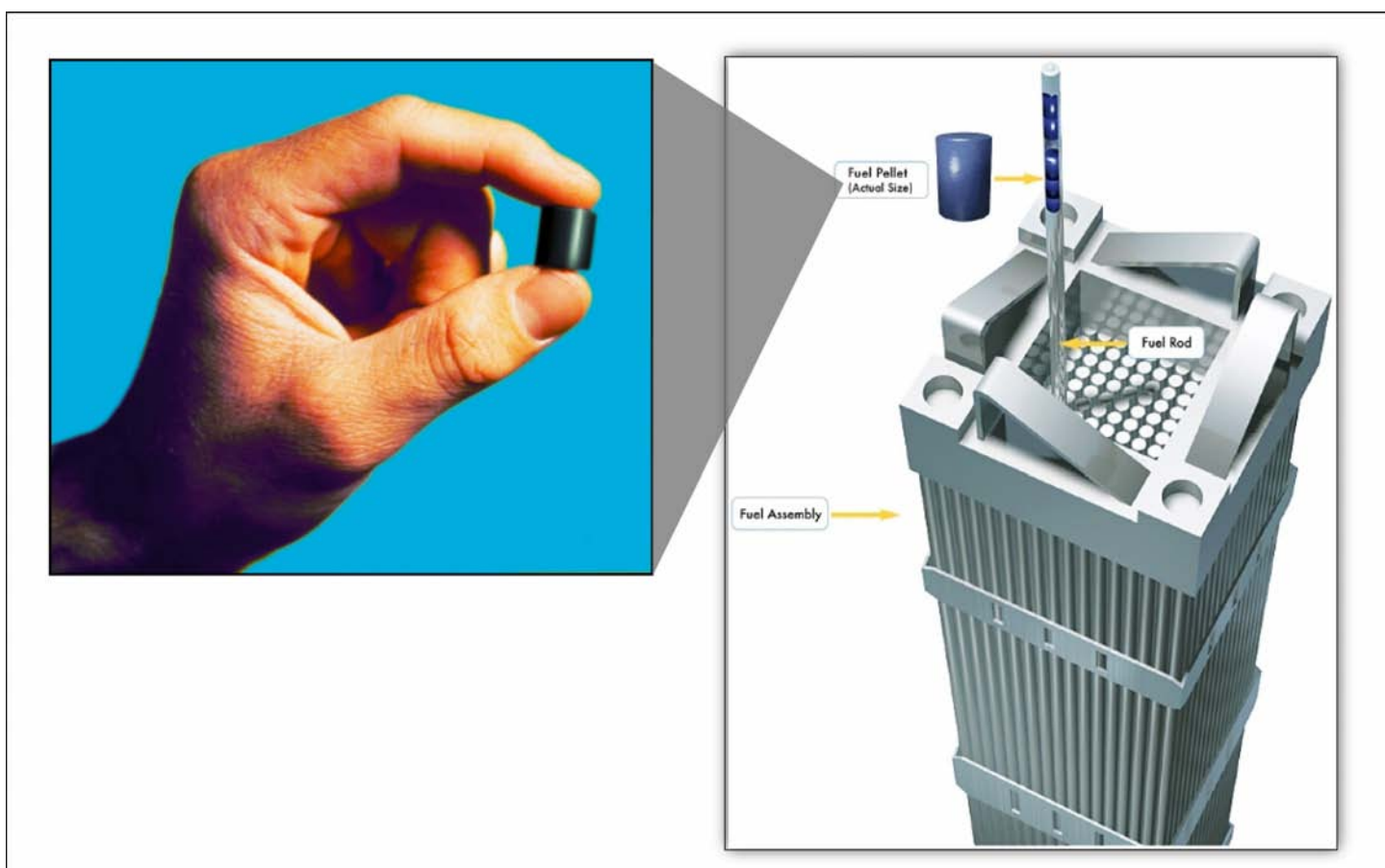
Figure 2: Fuel Pellet and Fuel Rod Assembly for a Commercial Nuclear Power Reactor
